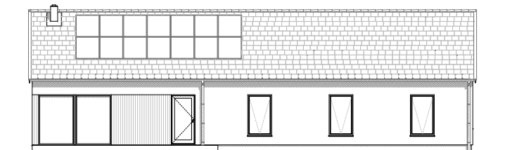
South Elevation
