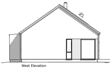
West Elevation
