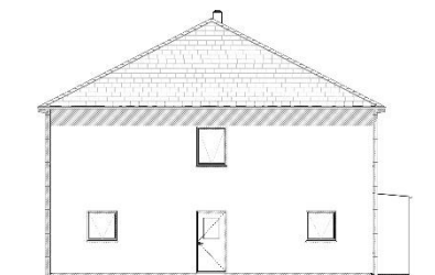
East Elevation
