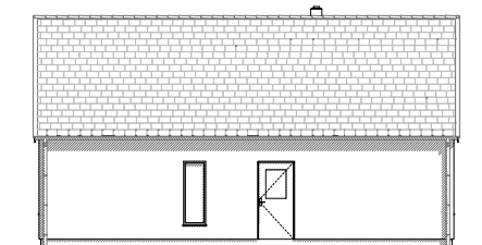
North Elevation
