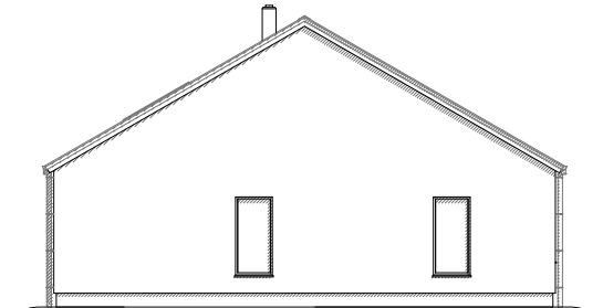
West Elevation
