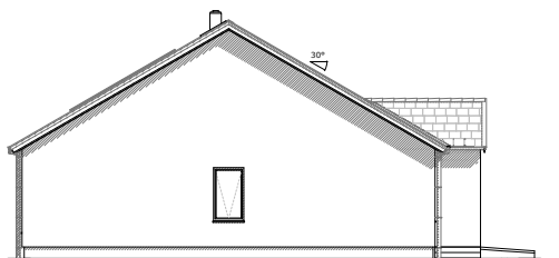
East Elevation
