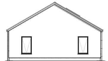
West elevation
