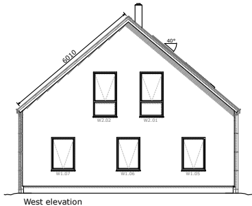
West elevation
