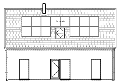
South elevation
