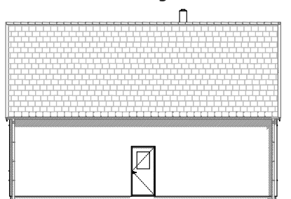
North elevation
