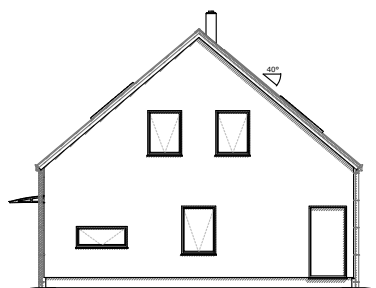
West elevation
