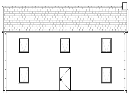
North Elevation
