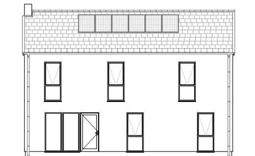
South Elevation
