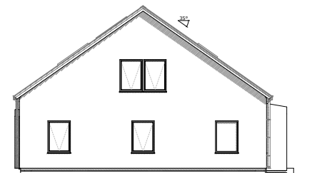
East Elevation
