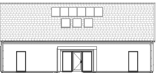
South Elevation
